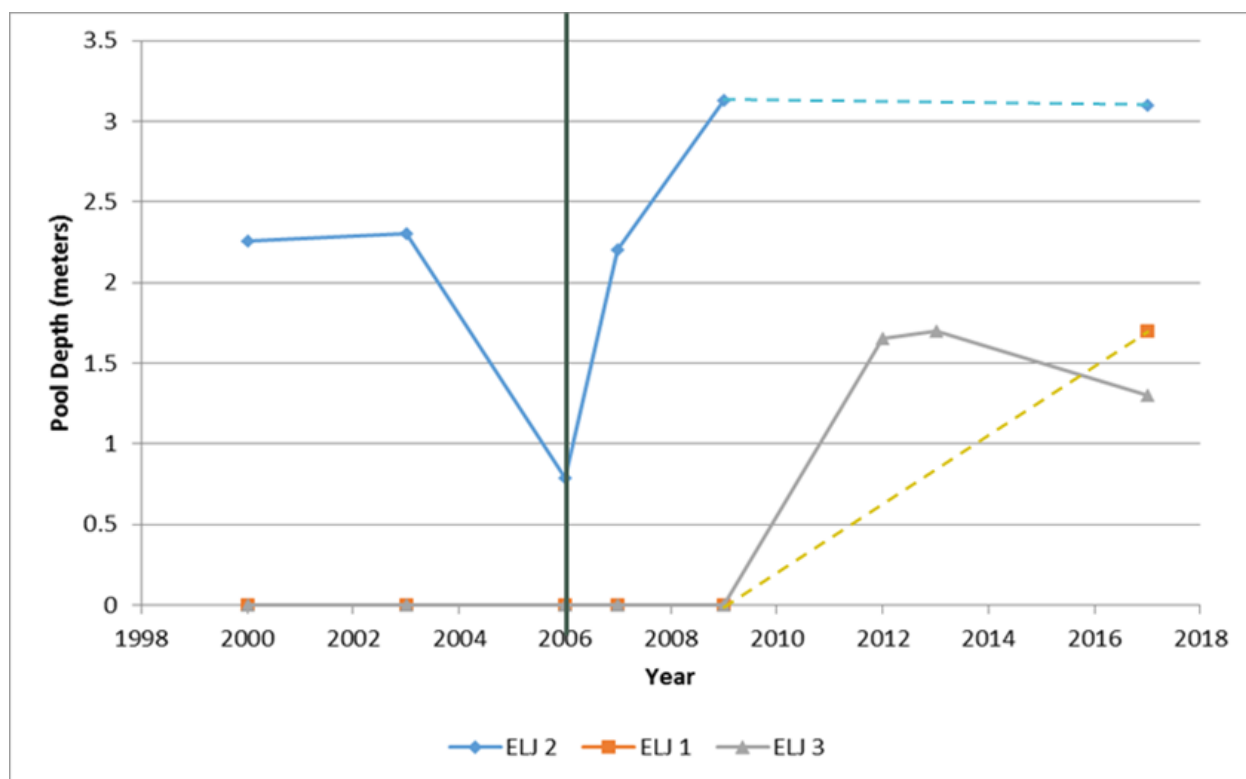
Figure 89: Pool development through time at the three engineered logjam sites in the Lower Hutchinson Creek Project.
