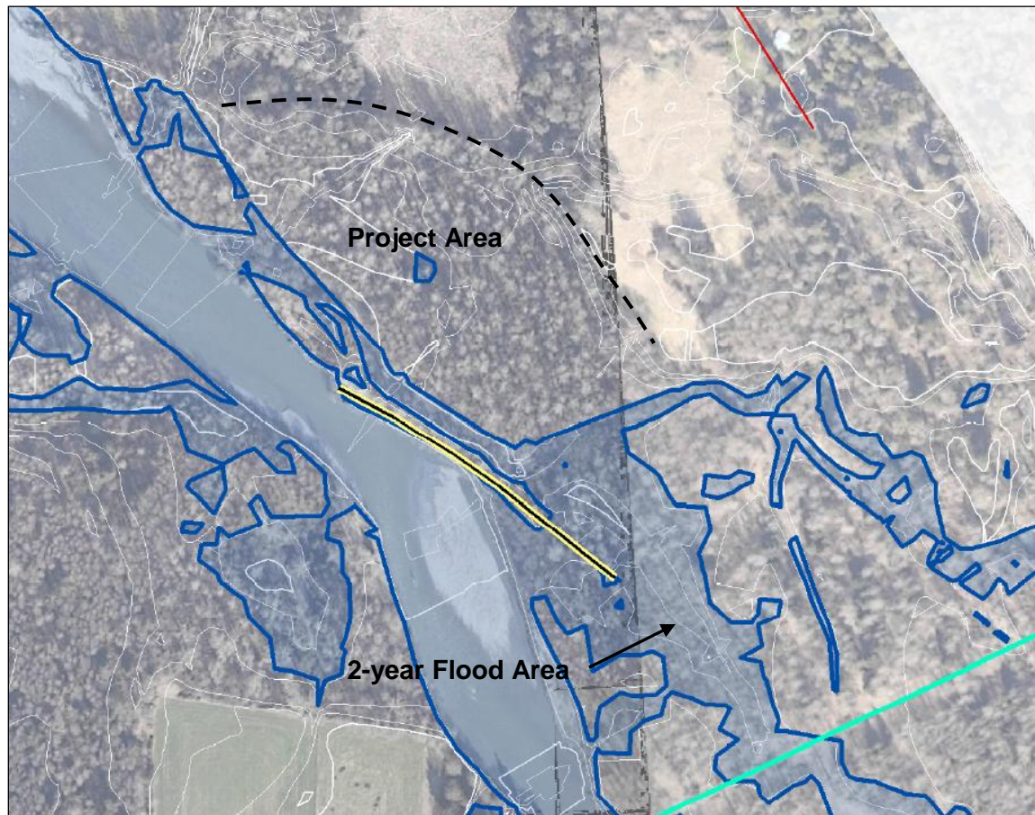
Figure 91: The 2-year flood inundation area based on the South Fork Nooksack HEC-RAS model at the project site before project construction.
