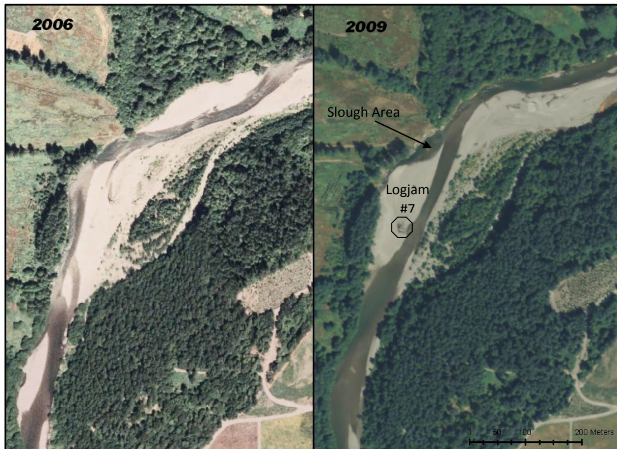
Figure 127: Looking downstream at the slough area before (left) and after (right) channel change.
