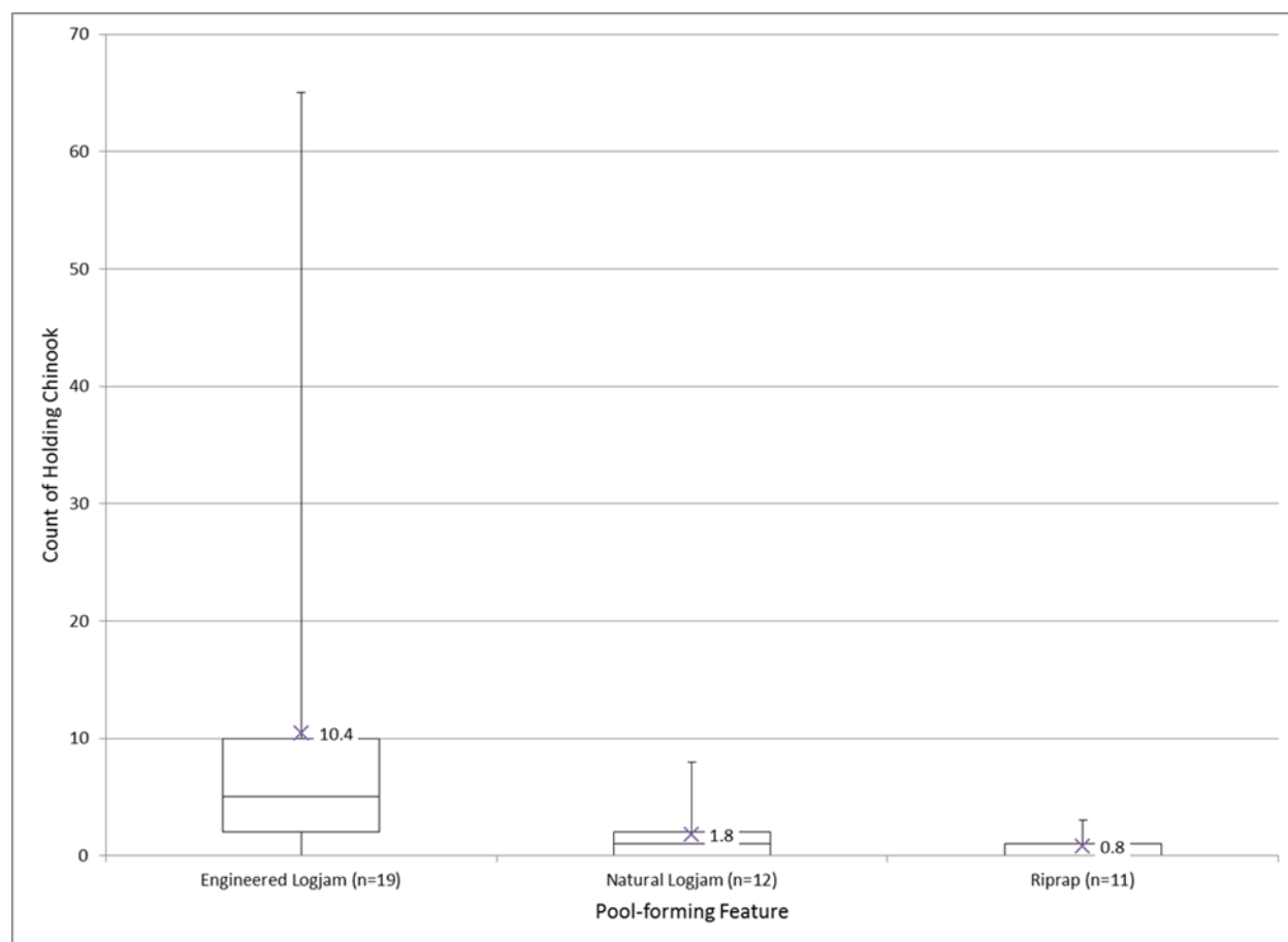
Figure 18: Adult holding chinook in pools by pool-forming feature (2017 data).
