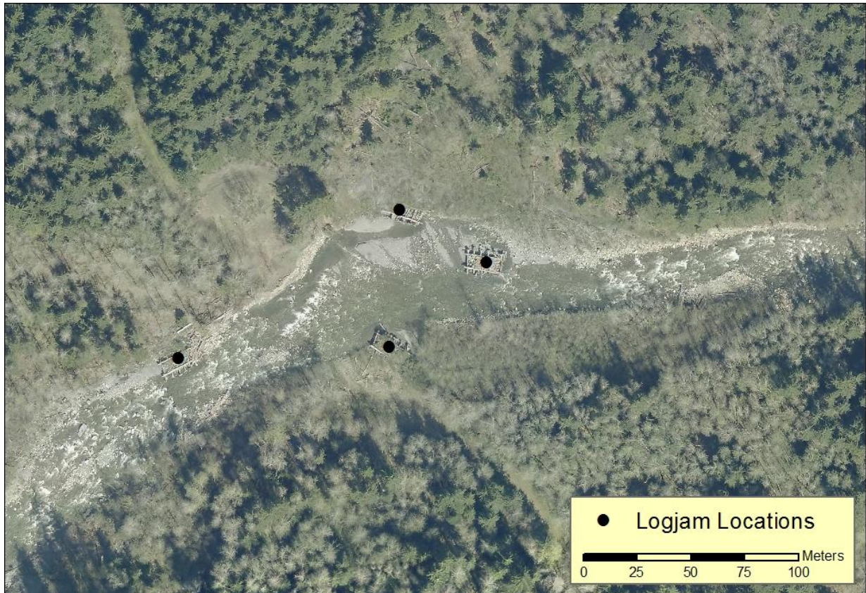
Figure 54: Habitat structures in the RM 30 project reach.
