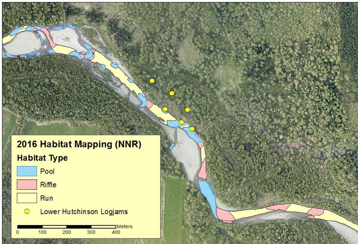
Figure 88: 2016 Habitat mapping showing the three pools formed by the three engineered logjams along the river (NNR data).
