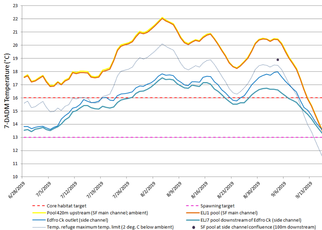
Figure 68. South Fork main channel and side channel temperature above and below the Edfro Creek confluence (paired probe controls) recorded in 2019 and presented as 7-day average maximum temperatures (LNR 2019).
