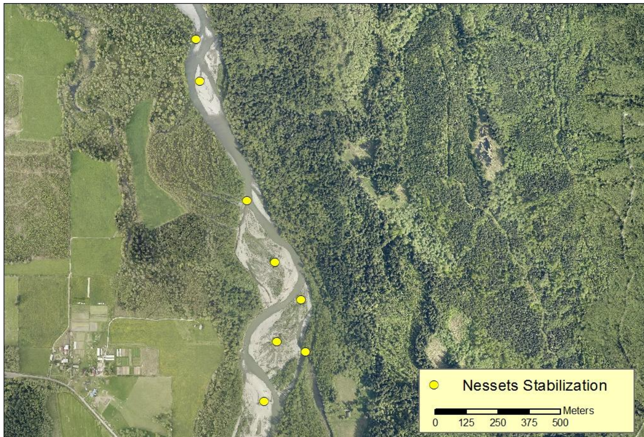
Figure 79: Nesset's LWD stabilization sites.
