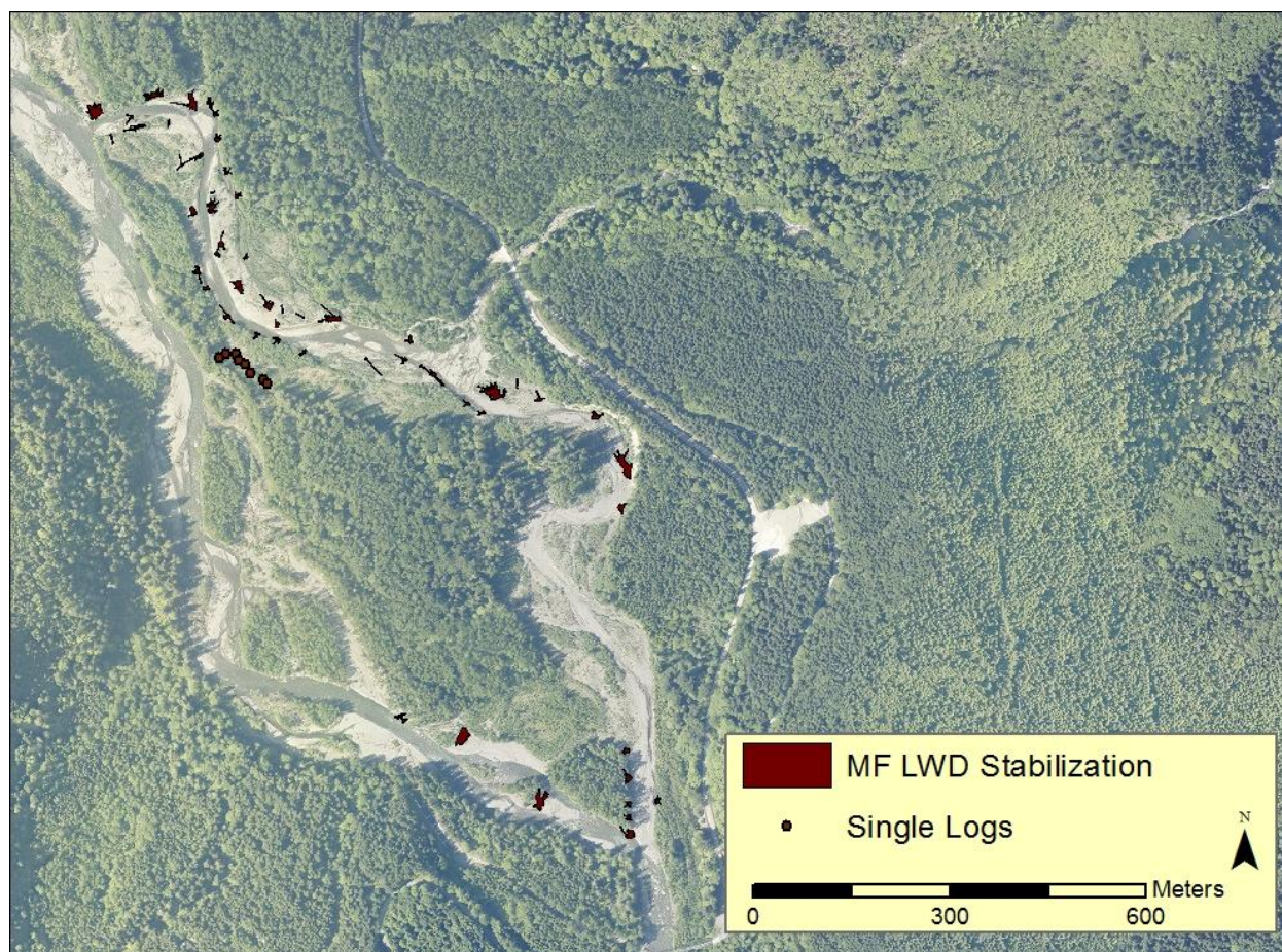
Figure 139: NSEA Middle Fork Nooksack LWD stabilization sites
