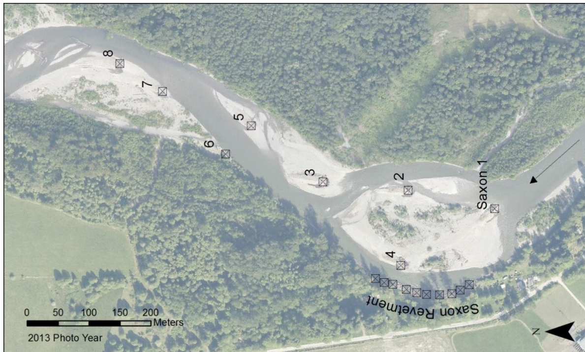
Figure 76: Saxon Reach Project showing Site ID for temperature monitoring.
