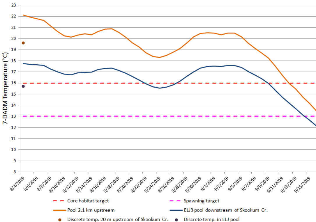
Figure 72. South Fork main channel temperature above and below the Skookum Creek confluence (paired probe controls) recorded in 2019 and presented as 7-day average maximum temperatures (7-DADM)(LNR 2019).
