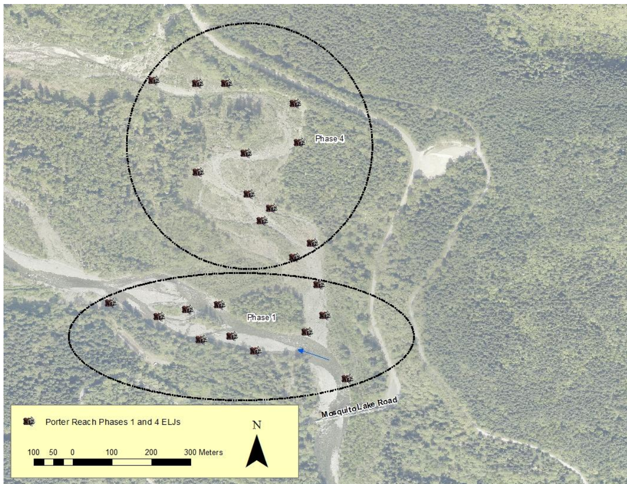
Figure 138: Phases 1 and 4 Middle Fork Porter Reach logjam locations.
