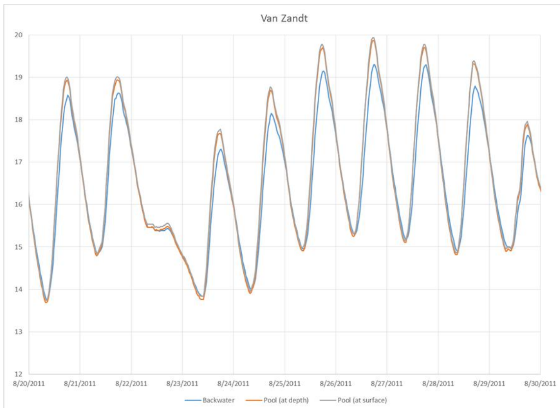
Figure 136: Continuous temperature monitoring in the pool associated with the stabilized cottonwood (Structure #15) showing temperature at the surface and bottom of the pool and in a backwater area (NNR data from 2011).
